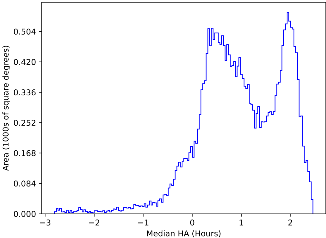
too_elab_r16_d2_ugrizy_v3.4_10yrs All sky z band: Median HA
