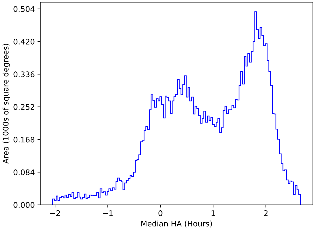
too_elab_r16_d2_ugrizy_v3.4_10yrs All sky u band: Median HA
