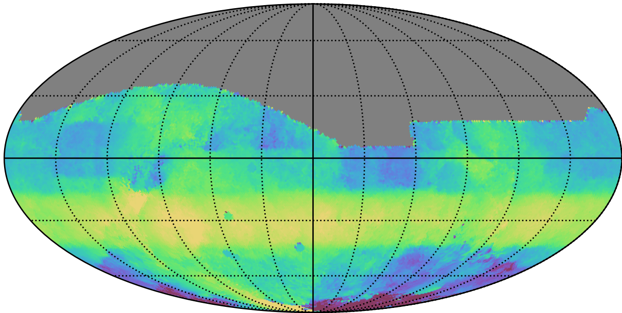
too_elab_r16_d2_ugrizy_v3.4_10yrs All sky r band: Median HA
