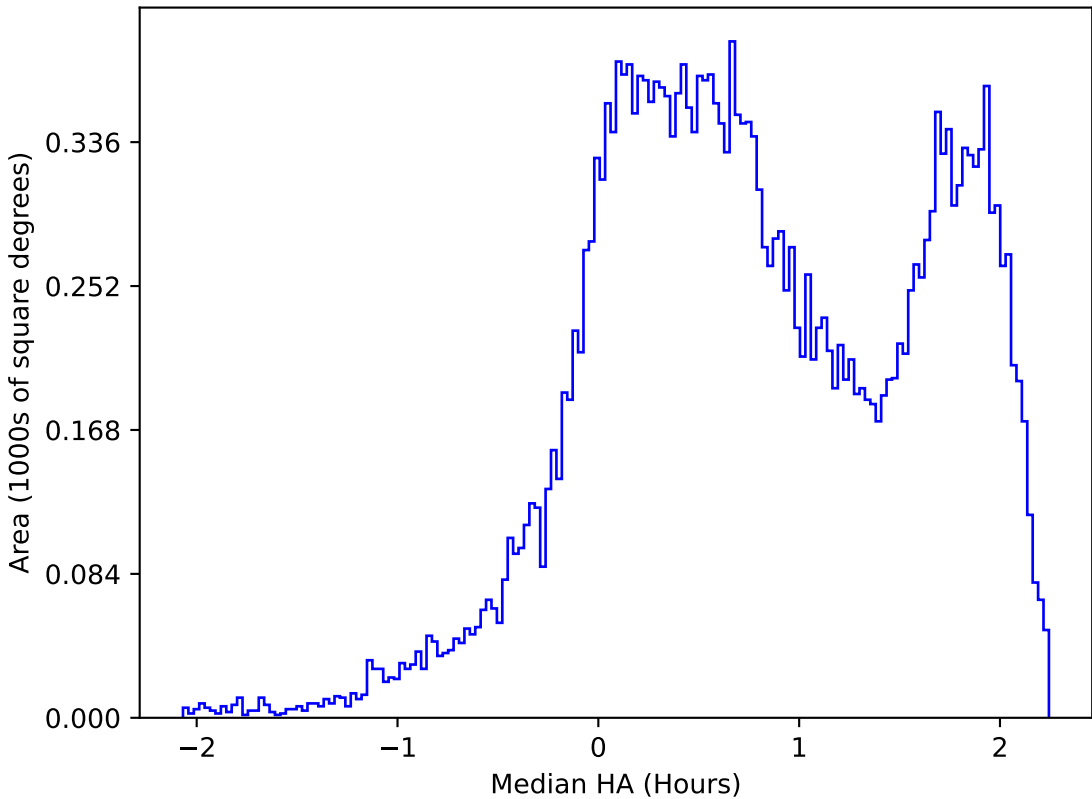
too_elab_r16_d2_ugrizy_v3.4_10yrs All sky r band: Median HA
