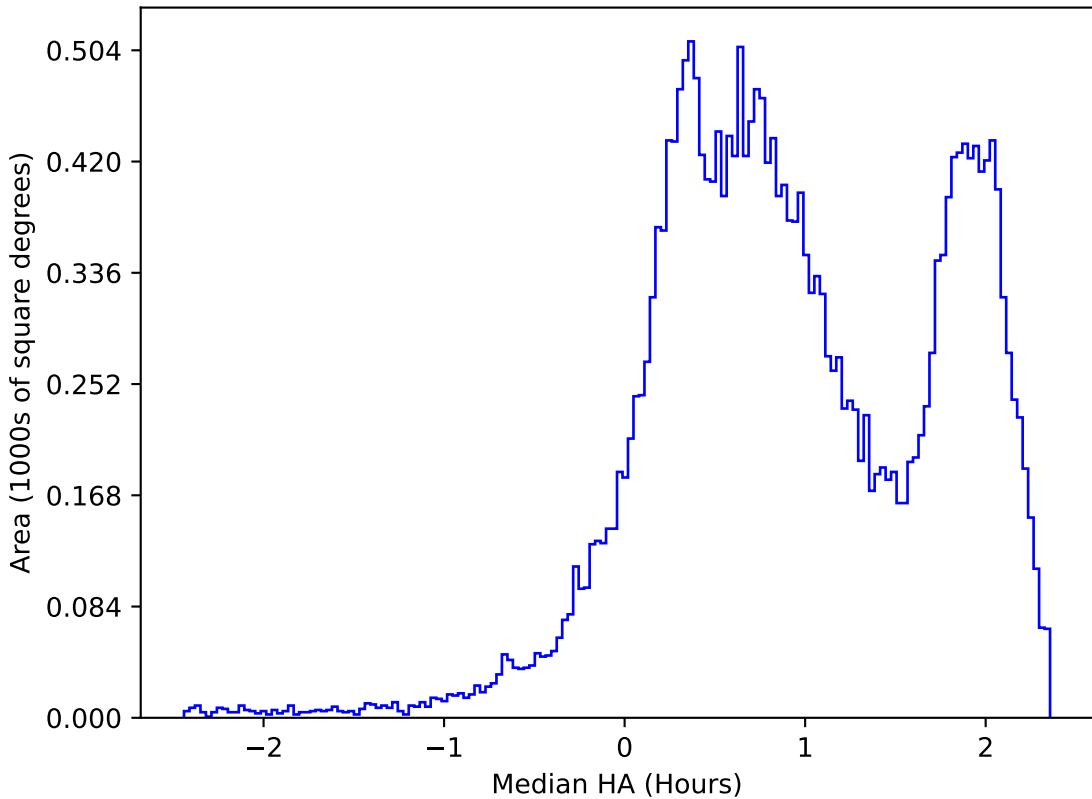
too_elab_r16_d2_ugrizy_v3.4_10yrs All sky i band: Median HA
