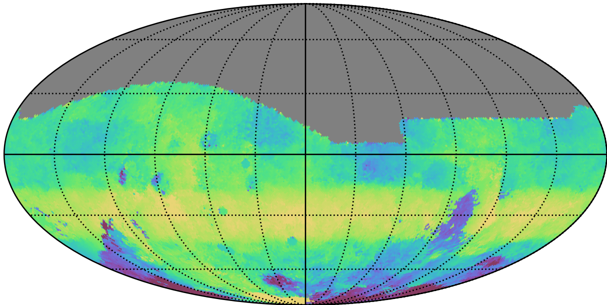
too_elab_r16_d2_ugrizy_v3.4_10yrs All sky g band: Median HA
