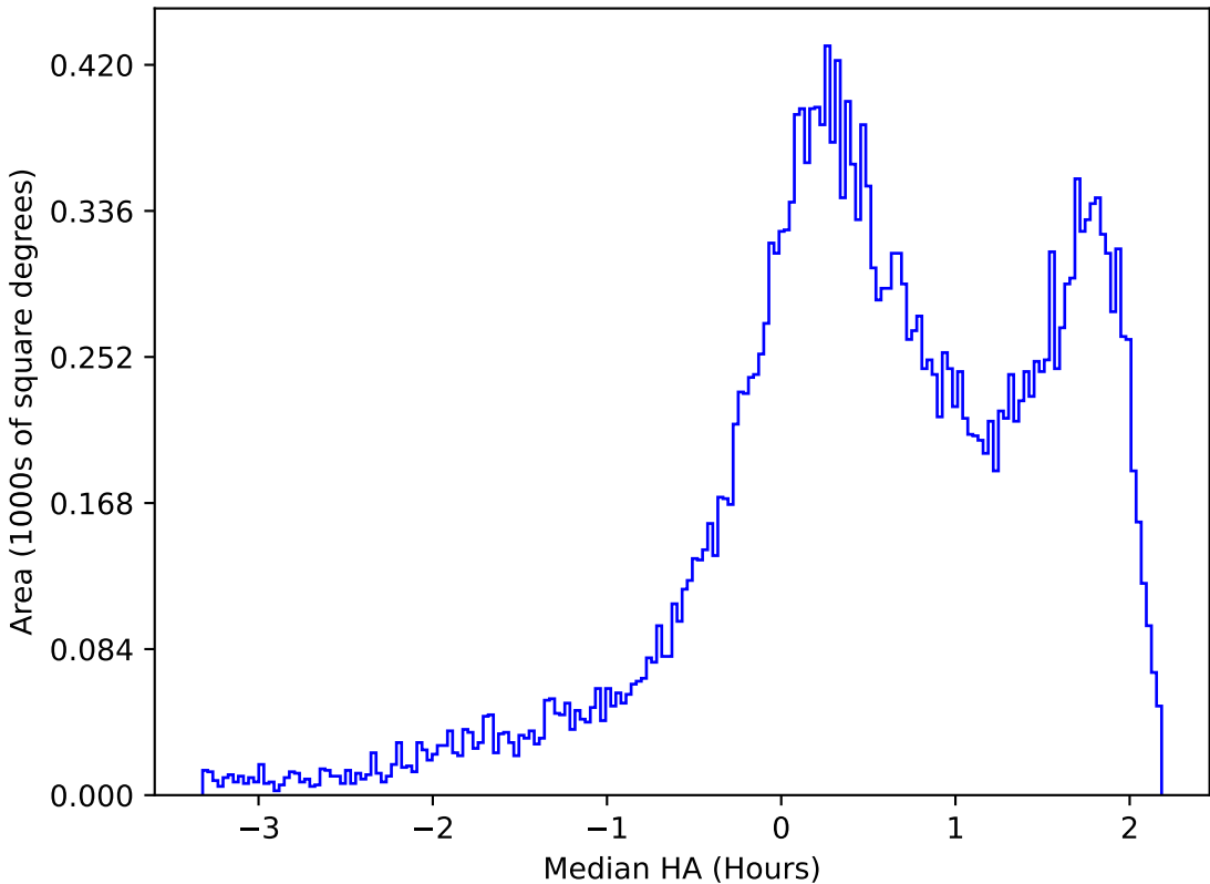
too_elab_r16_d2_ugrizy_v3.4_10yrs All sky g band: Median HA
