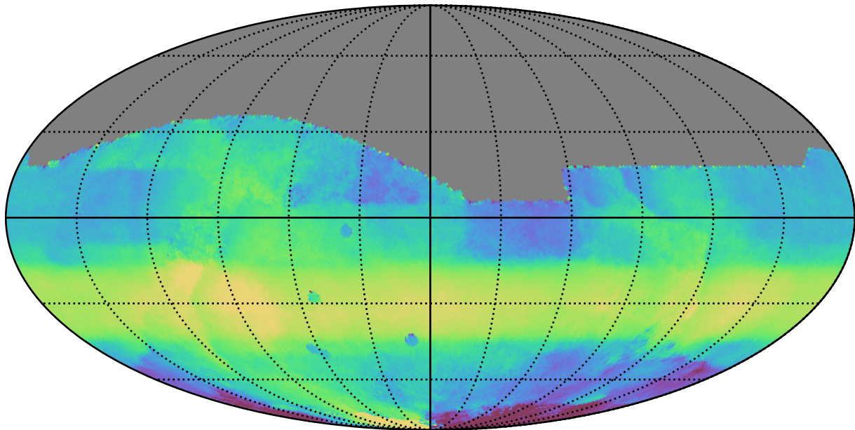
too_elab_r16_d2_ugrizy_v3.4_10yrs All sky all bands: Median HA
