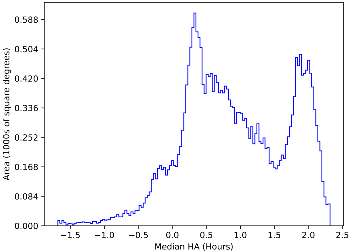
too_elab_r16_d2_ugrizy_v3.4_10yrs All sky all bands: Median HA
