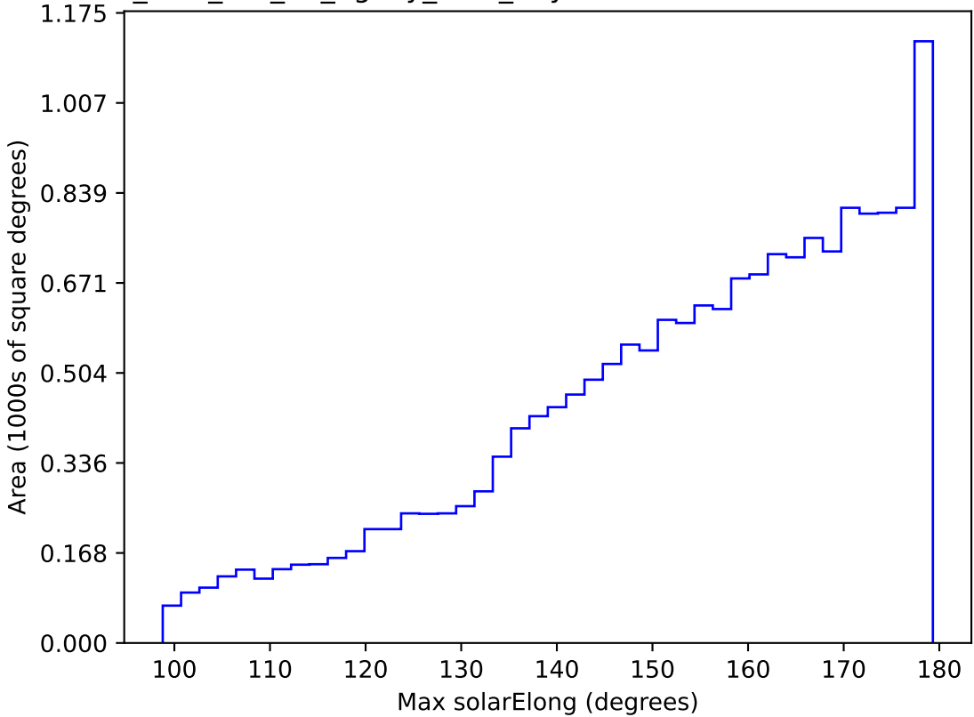
too_elab_r16_d2_ugrizy_v3.4_10yrs WFD z band: Max solarElong
