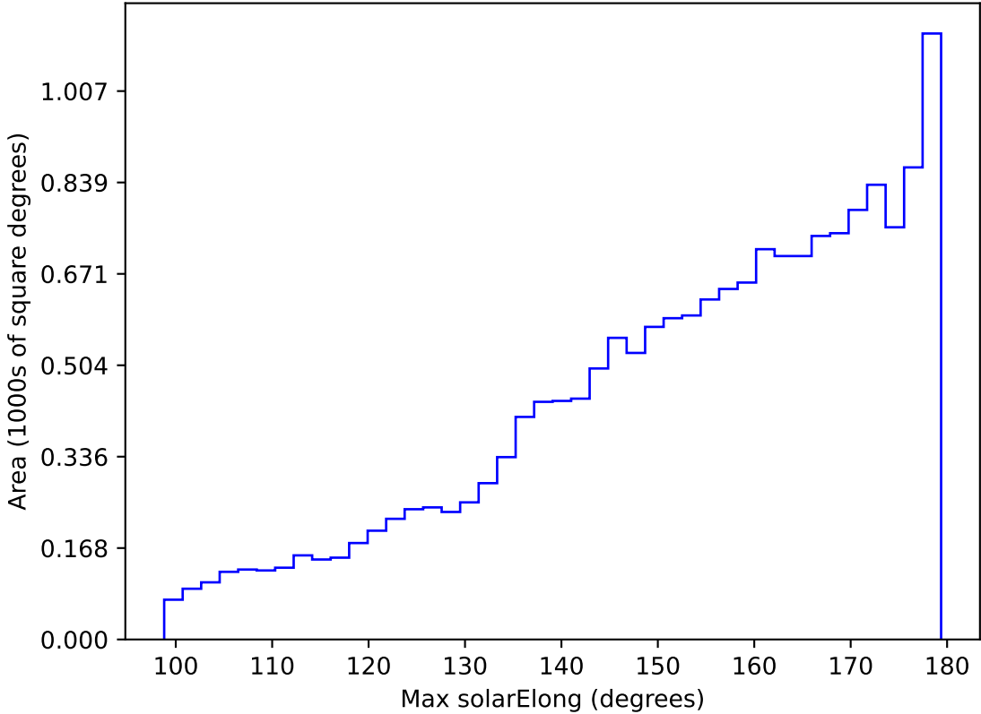
too_elab_r16_d2_ugrizy_v3.4_10yrs WFD r band: Max solarElong
