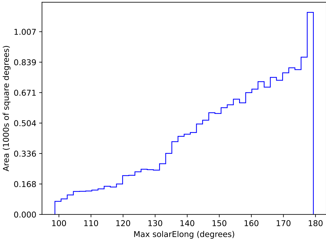
too_elab_r16_d2_ugrizy_v3.4_10yrs WFD i band: Max solarElong
