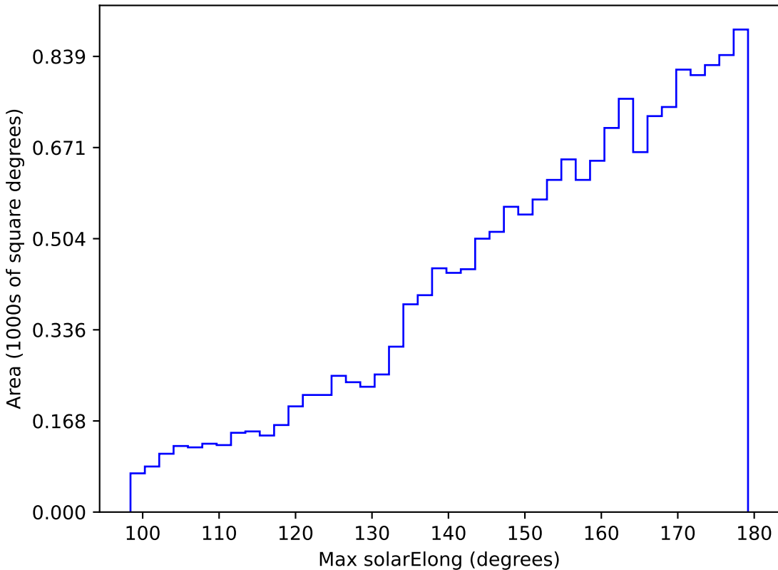
too_elab_r16_d2_ugrizy_v3.4_10yrs WFD g band: Max solarElong
