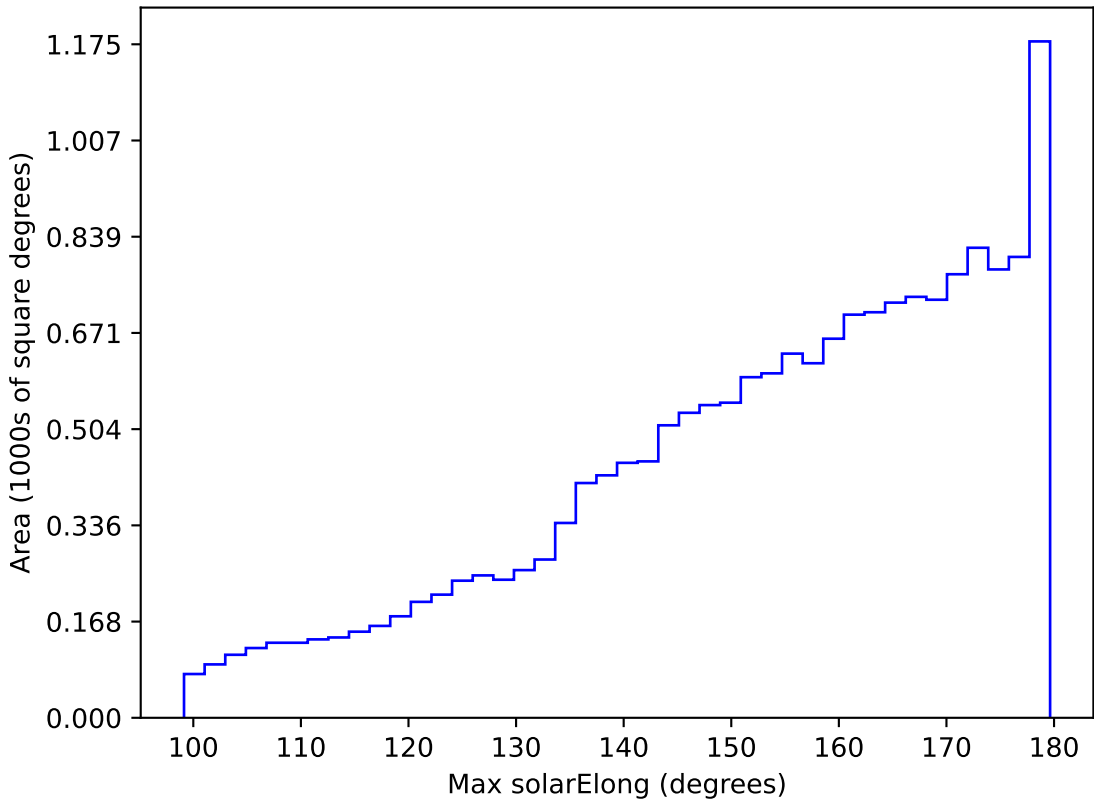
too_elab_r16_d2_ugrizy_v3.4_10yrs WFD all bands: Max solarElong
