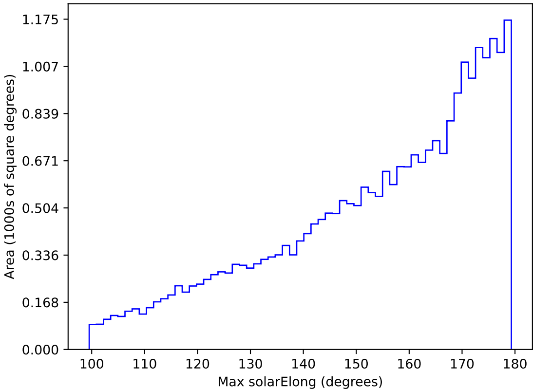
too_elab_r16_d2_ugrizy_v3.4_10yrs All sky z band: Max solarElong
