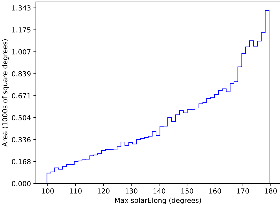
too_elab_r16_d2_ugrizy_v3.4_10yrs All sky r band: Max solarElong
