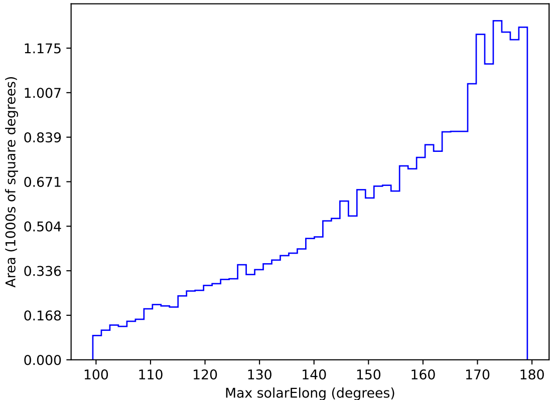
too_elab_r16_d2_ugrizy_v3.4_10yrs All sky g band: Max solarElong
