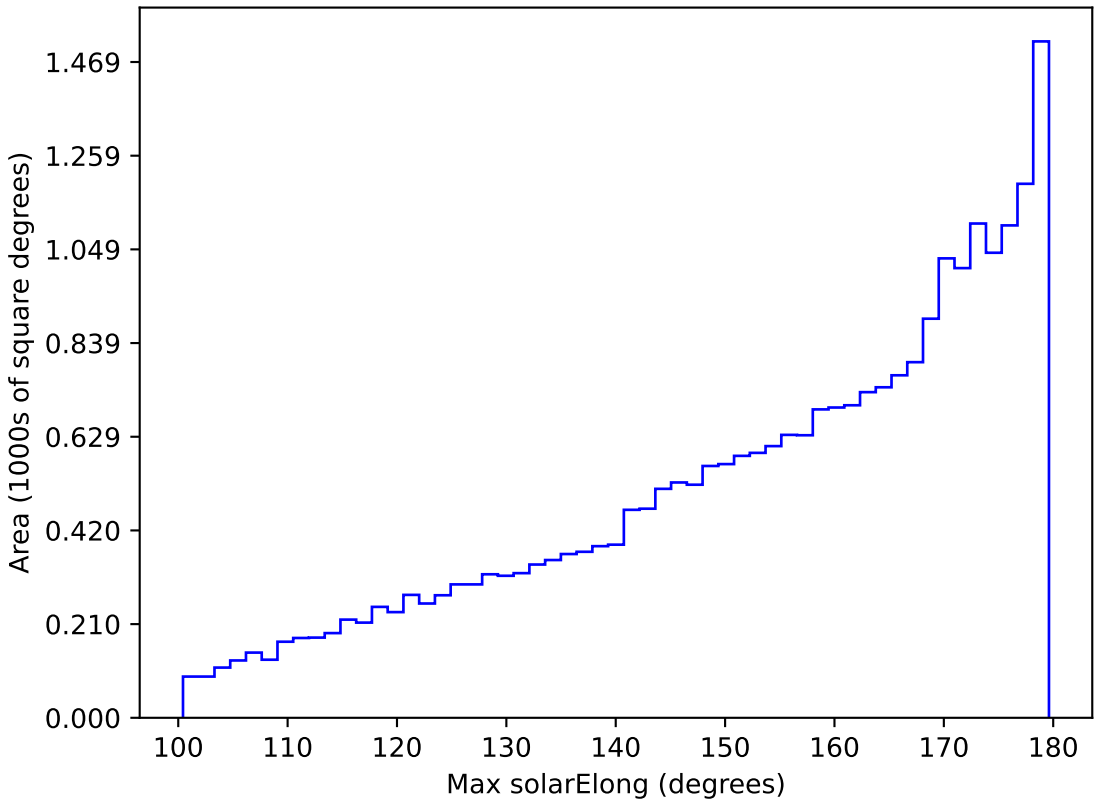
too_elab_r16_d2_ugrizy_v3.4_10yrs All sky all bands: Max solarElong
