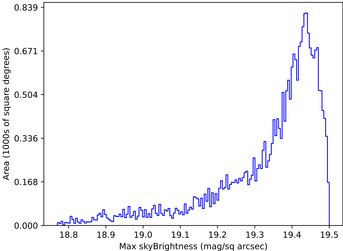
too_elab_r16_d2_ugrizy_v3.4_10yrs Yr 1 z band: Max skyBrightness
