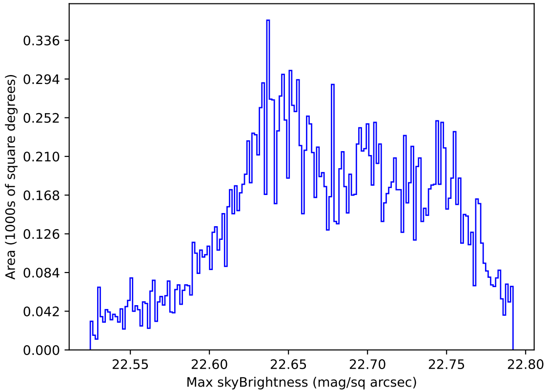
too_elab_r16_d2_ugrizy_v3.4_10yrs Yr 1 u band: Max skyBrightness
