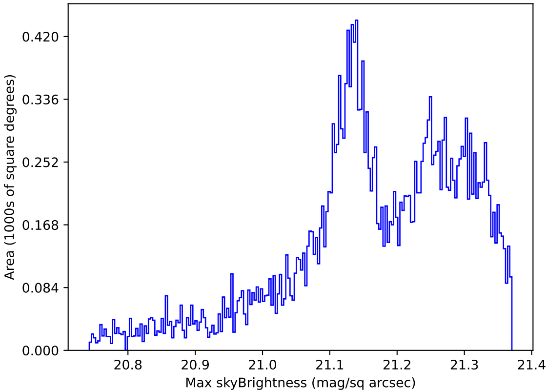
too_elab_r16_d2_ugrizy_v3.4_10yrs Yr 1 r band: Max skyBrightness
