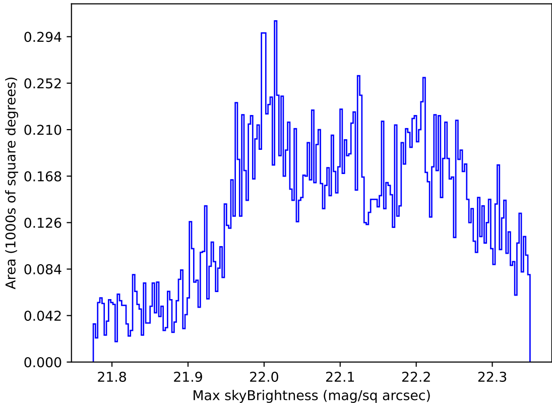
too_elab_r16_d2_ugrizy_v3.4_10yrs Yr 1 g band: Max skyBrightness
