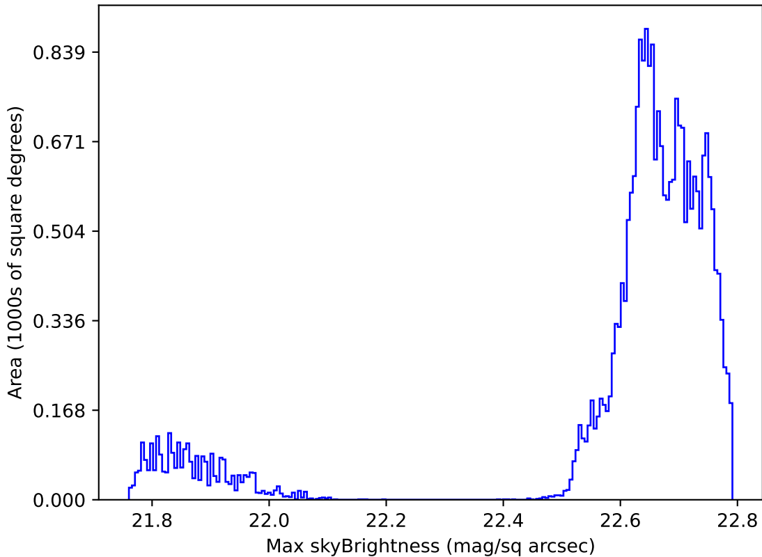
too_elab_r16_d2_ugrizy_v3.4_10yrs Yr 1 all bands: Max skyBrightness
