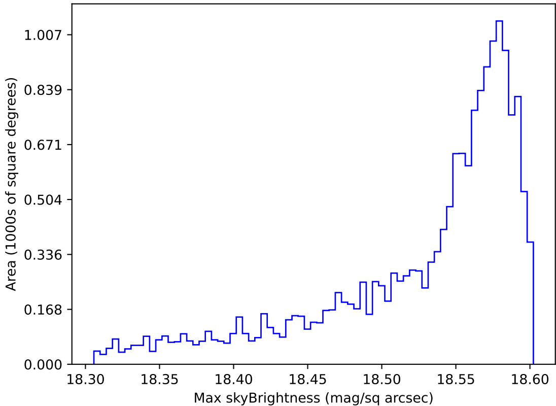
too_elab_r16_d2_ugrizy_v3.4_10yrs WFD y band: Max skyBrightness
