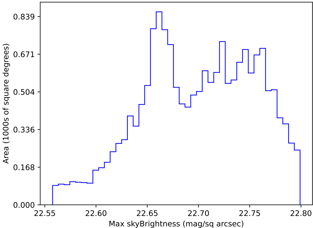
too_elab_r16_d2_ugrizy_v3.4_10yrs WFD u band: Max skyBrightness
