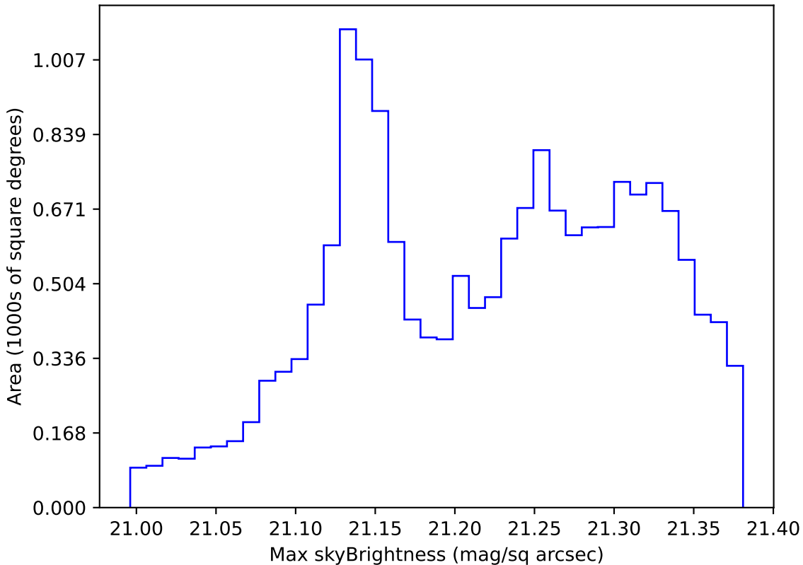
too_elab_r16_d2_ugrizy_v3.4_10yrs WFD r band: Max skyBrightness
