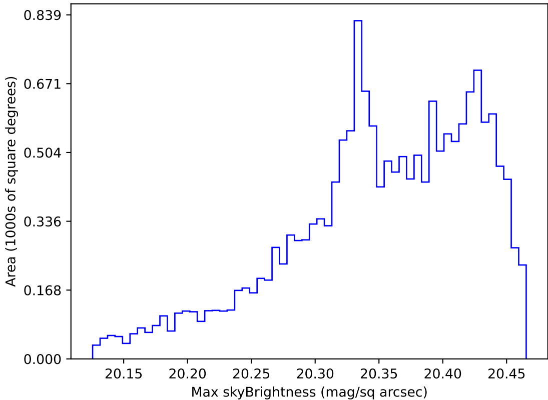
too_elab_r16_d2_ugrizy_v3.4_10yrs WFD i band: Max skyBrightness
