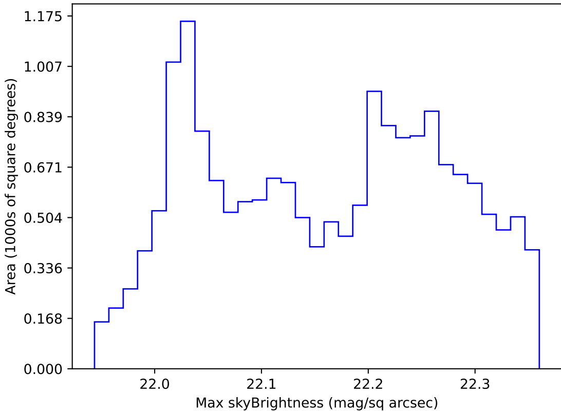
too_elab_r16_d2_ugrizy_v3.4_10yrs WFD g band: Max skyBrightness
