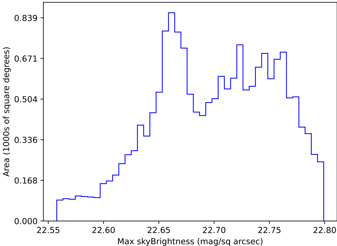
too_elab_r16_d2_ugrizy_v3.4_10yrs WFD all bands: Max skyBrightness
