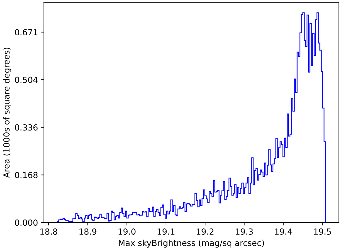
too_elab_r16_d2_ugrizy_v3.4_10yrs All sky z band: Max skyBrightness
