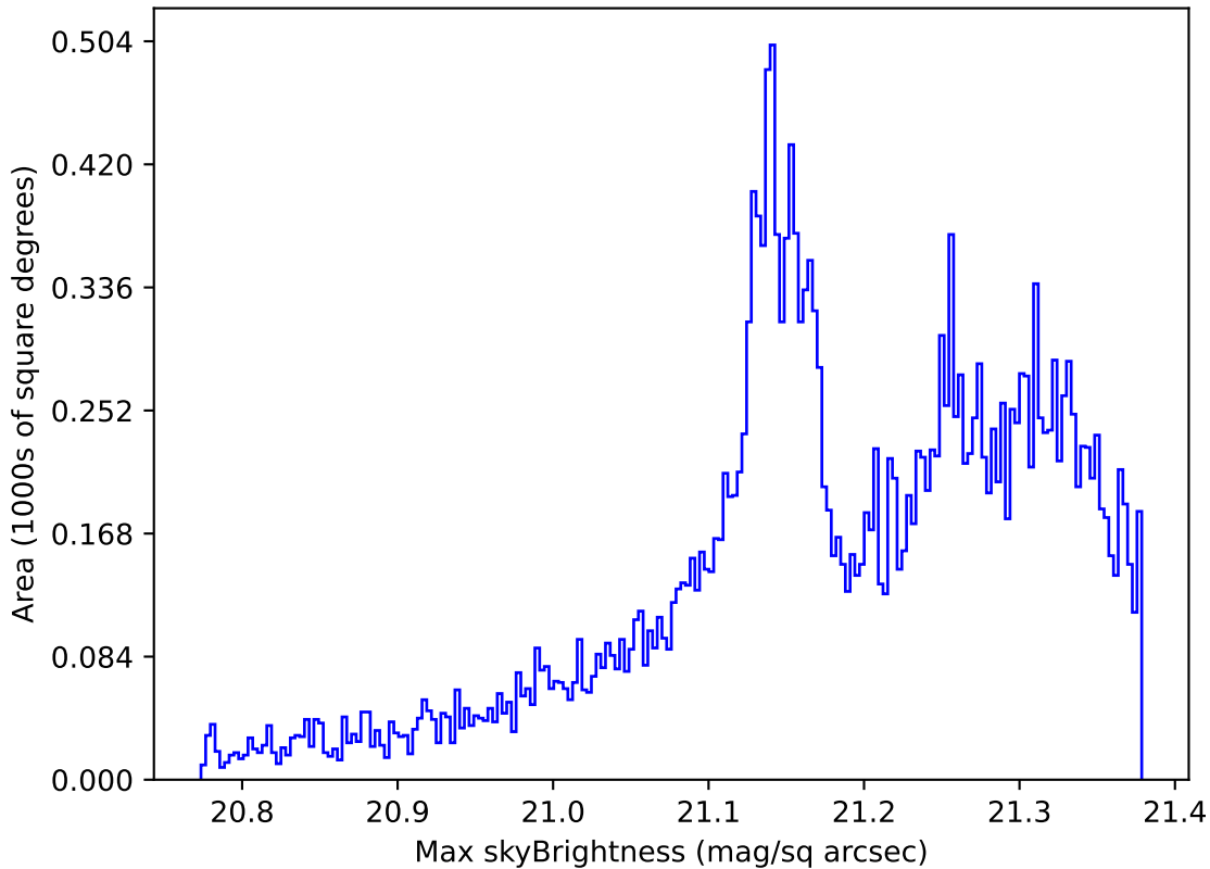
too_elab_r16_d2_ugrizy_v3.4_10yrs All sky r band: Max skyBrightness
