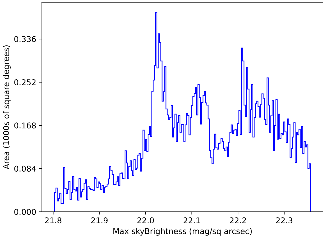
too_elab_r16_d2_ugrizy_v3.4_10yrs All sky g band: Max skyBrightness
