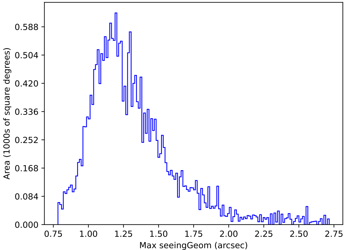
too_elab_r16_d2_ugrizy_v3.4_10yrs Yr 1 u band: Max seeingGeom
