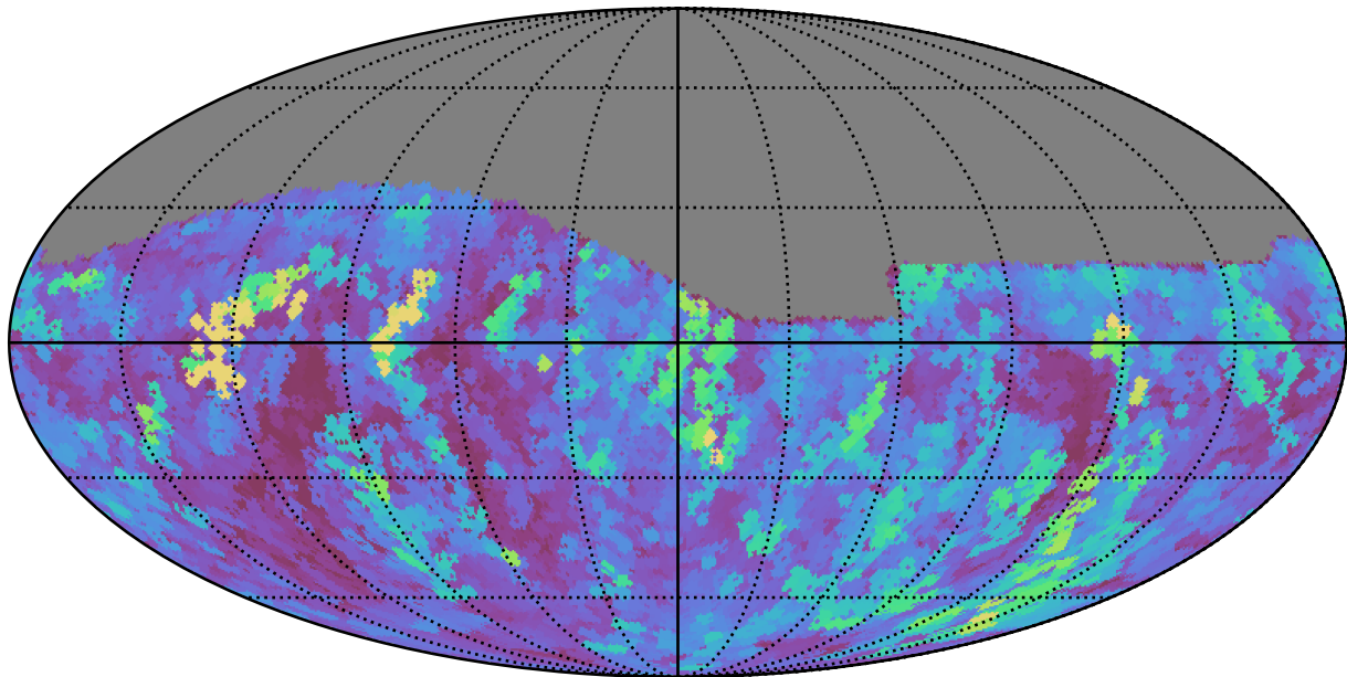
too_elab_r16_d2_ugrizy_v3.4_10yrs Yr 1 r band: Max seeingGeom
