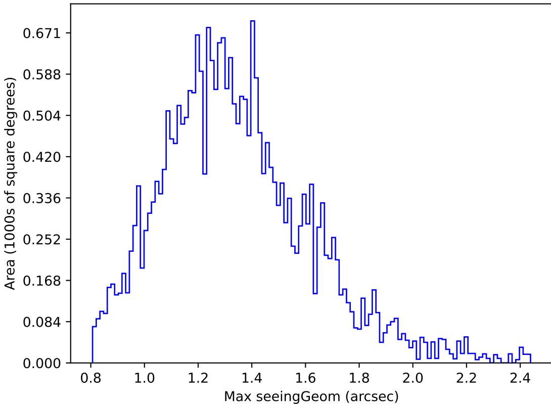
too_elab_r16_d2_ugrizy_v3.4_10yrs Yr 1 r band: Max seeingGeom
