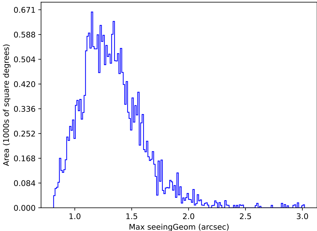
too_elab_r16_d2_ugrizy_v3.4_10yrs Yr 1 g band: Max seeingGeom
