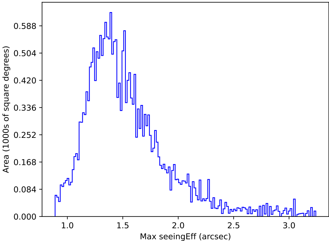
too_elab_r16_d2_ugrizy_v3.4_10yrs Yr 1 u band: Max seeingEff
