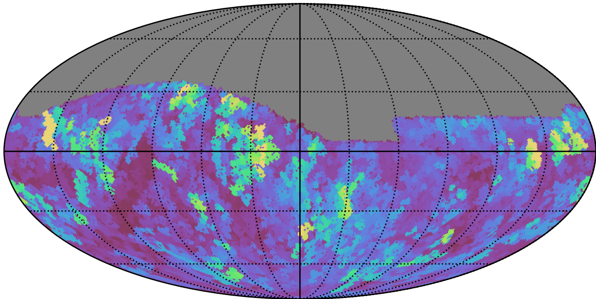
too_elab_r16_d2_ugrizy_v3.4_10yrs Yr 1 i band: Max seeingEff
