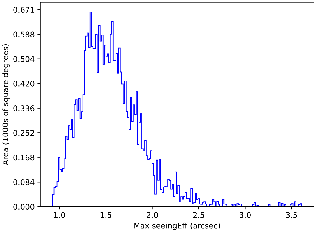
too_elab_r16_d2_ugrizy_v3.4_10yrs Yr 1 g band: Max seeingEff
