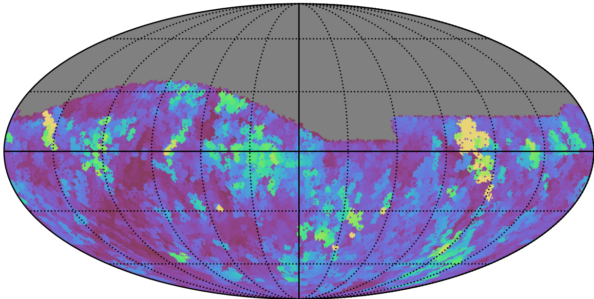
too_elab_r16_d2_ugrizy_v3.4_10yrs Yr 1 all bands: Max seeingEff
