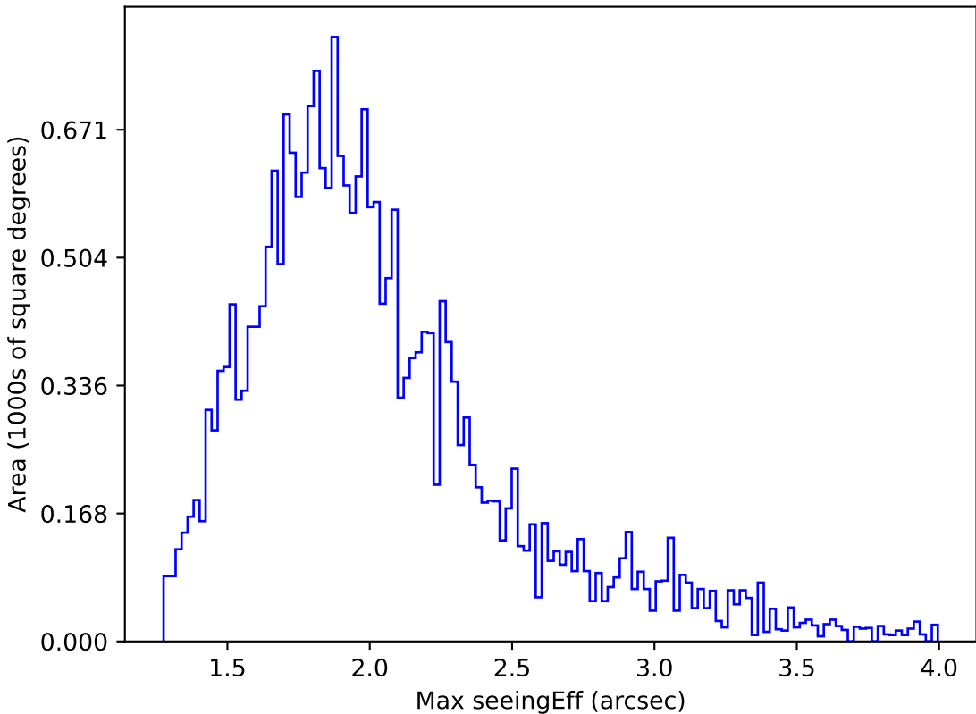
too_elab_r16_d2_ugrizy_v3.4_10yrs Yr 1 all bands: Max seeingEff
