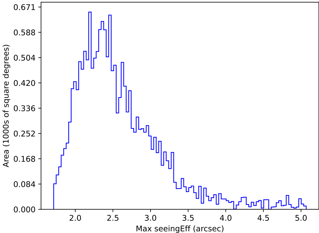
too_elab_r16_d2_ugrizy_v3.4_10yrs WFD z band: Max seeingEff
