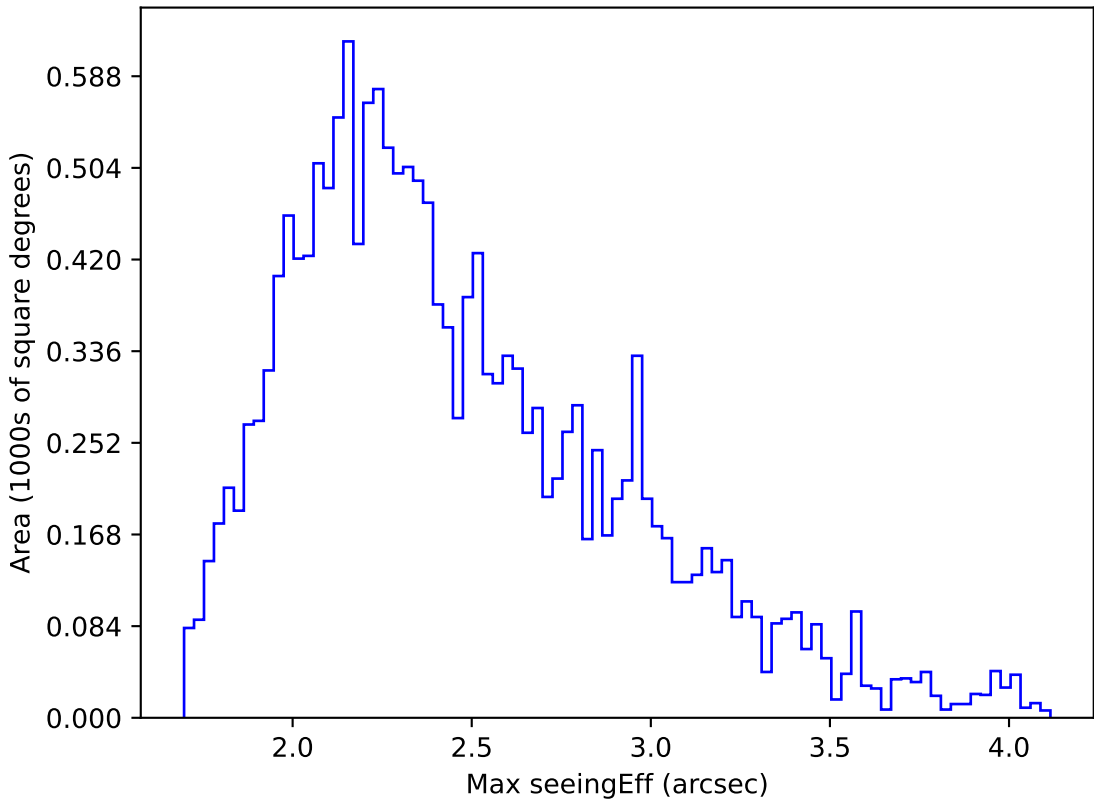
too_elab_r16_d2_ugrizy_v3.4_10yrs WFD u band: Max seeingEff
