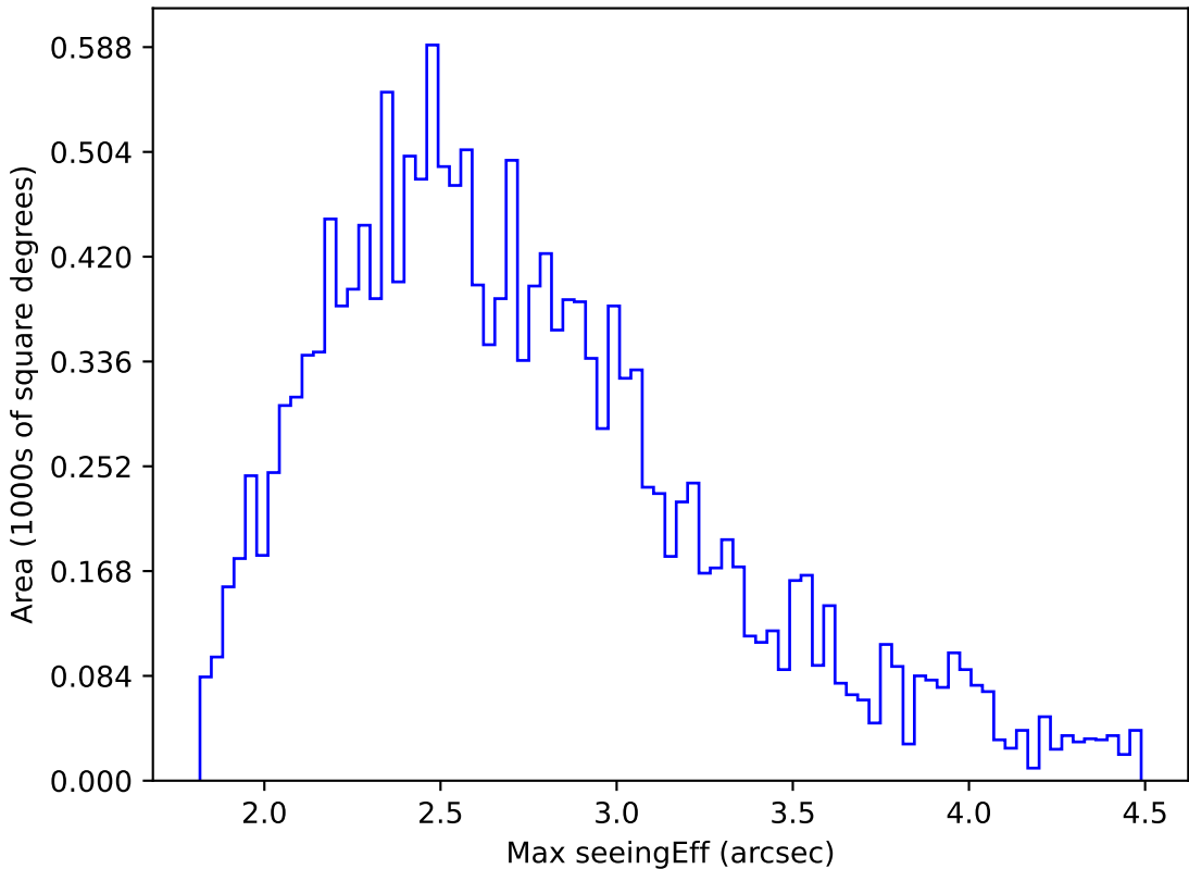
too_elab_r16_d2_ugrizy_v3.4_10yrs WFD r band: Max seeingEff
