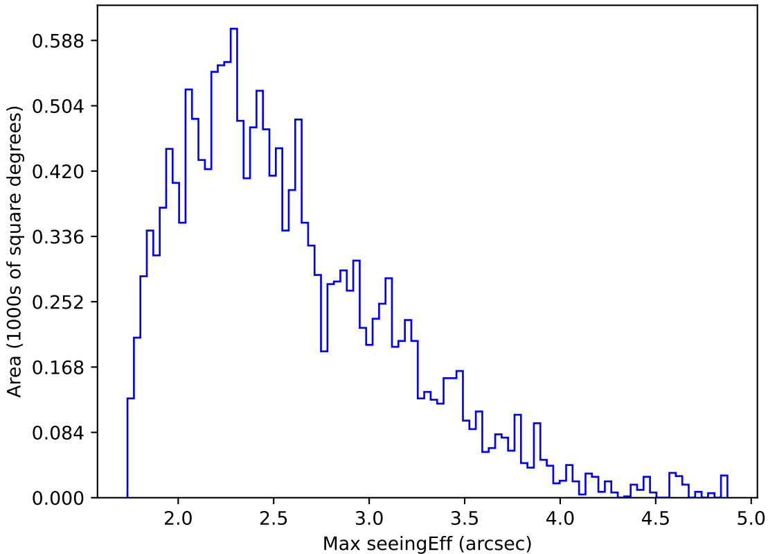
too_elab_r16_d2_ugrizy_v3.4_10yrs WFD g band: Max seeingEff
