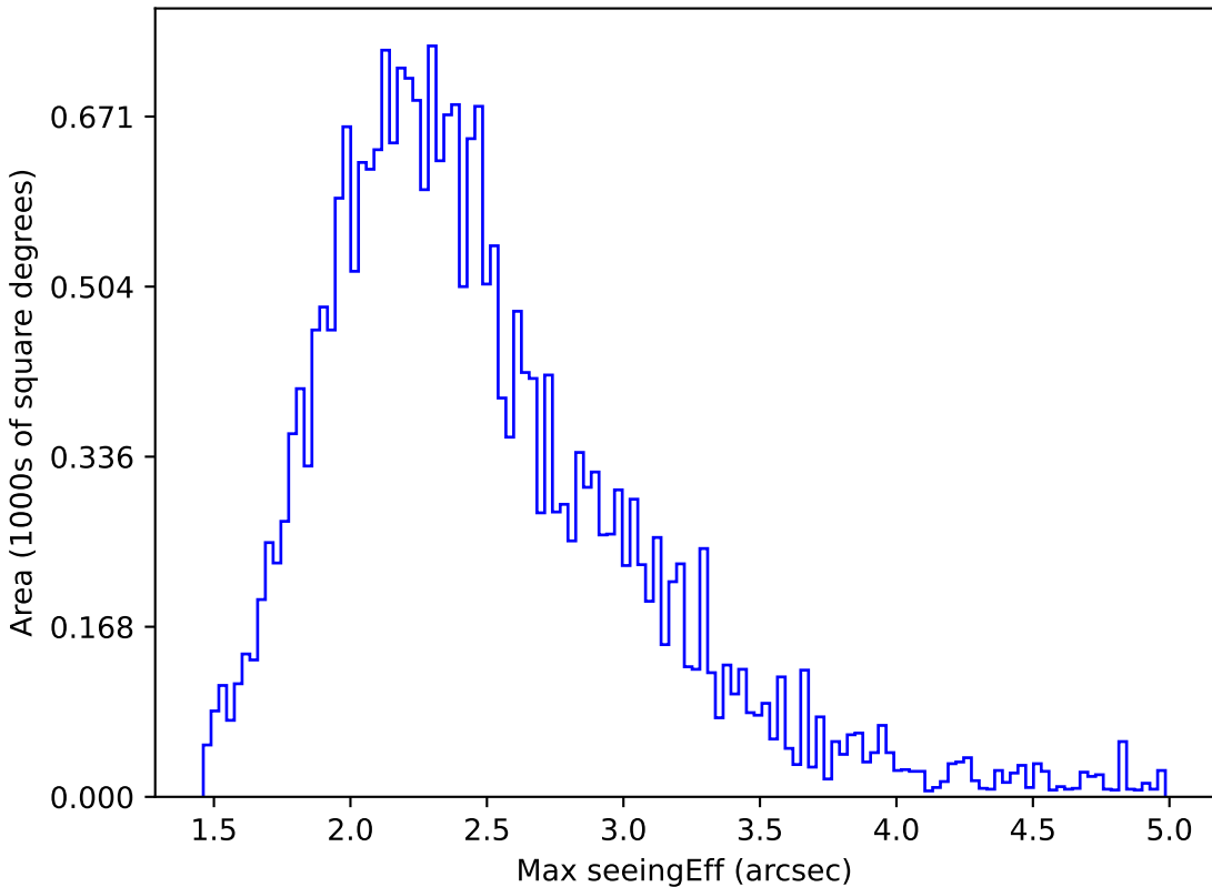
too_elab_r16_d2_ugrizy_v3.4_10yrs All sky z band: Max seeingEff
