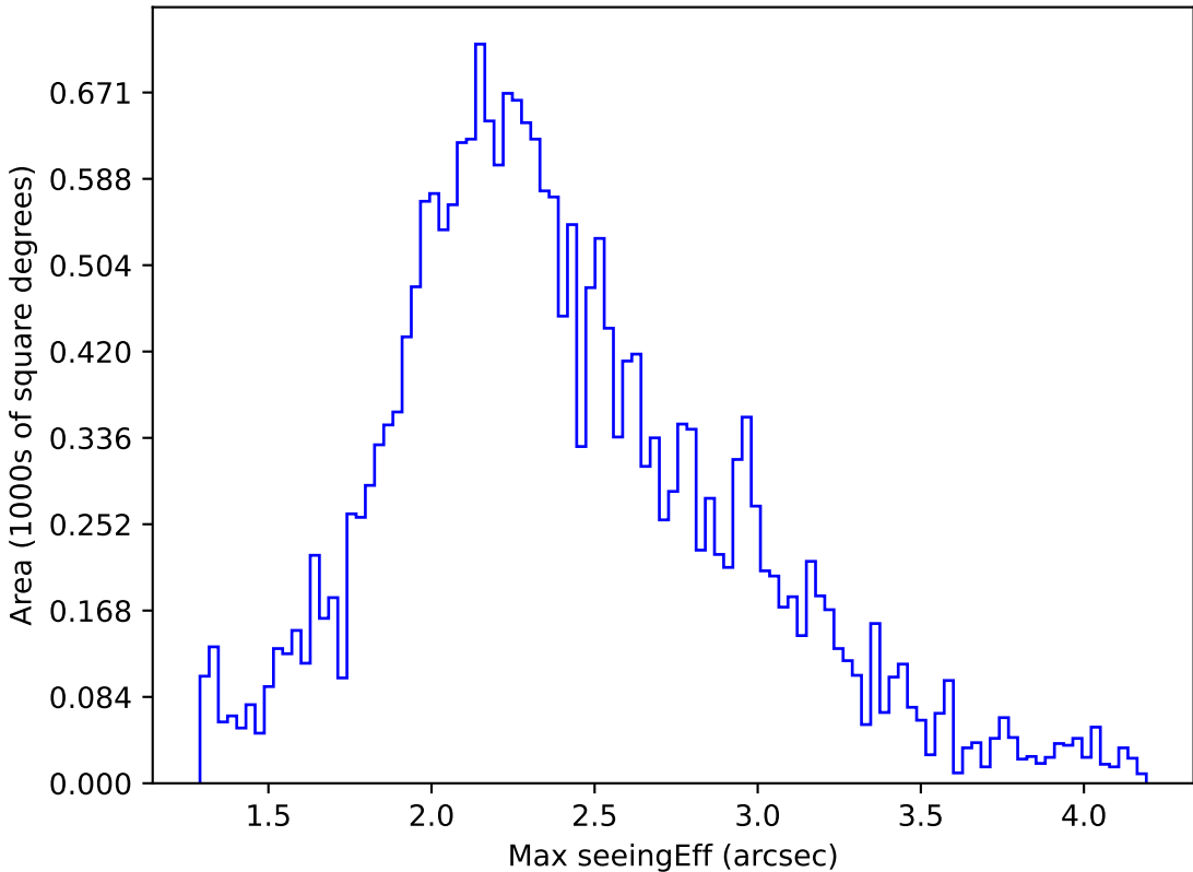
too_elab_r16_d2_ugrizy_v3.4_10yrs All sky u band: Max seeingEff
