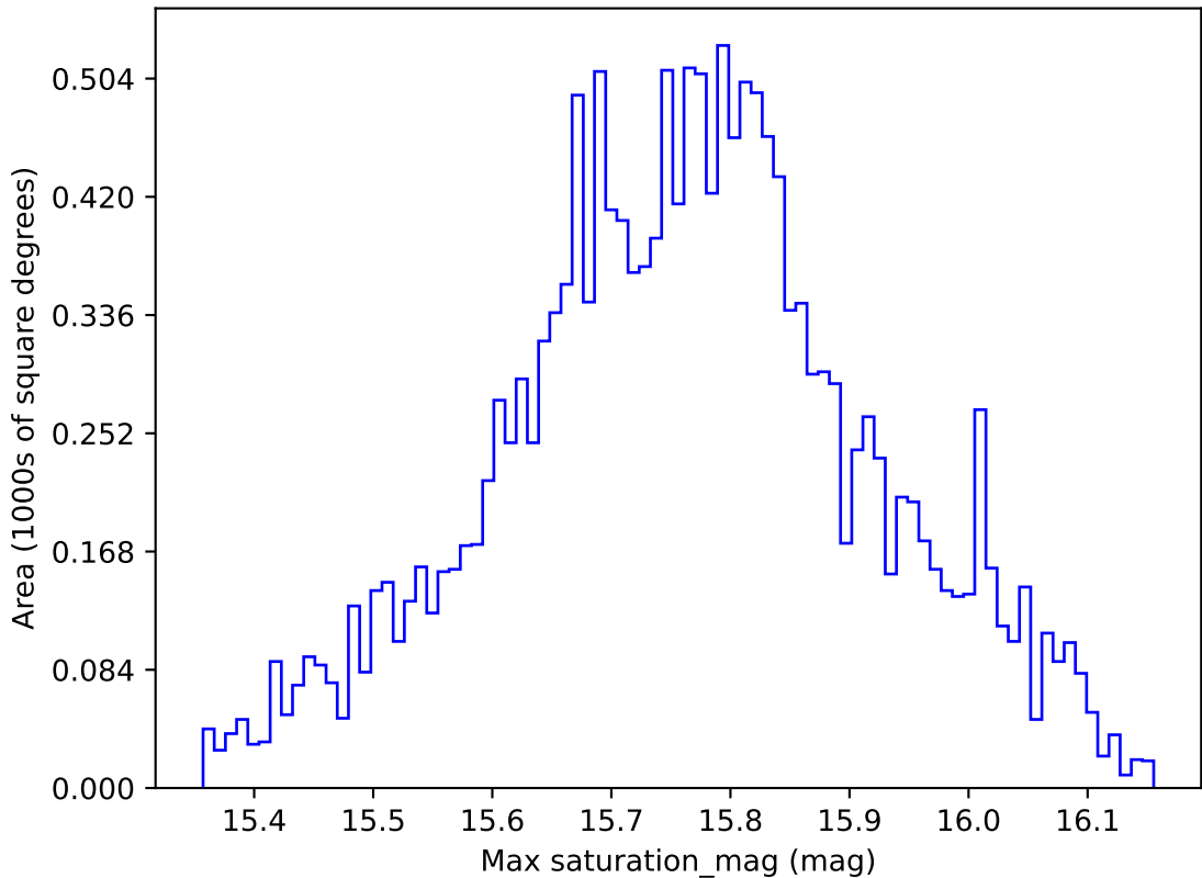
too_elab_r16_d2_ugrizy_v3.4_10yrs WFD r band: Max saturation_mag
