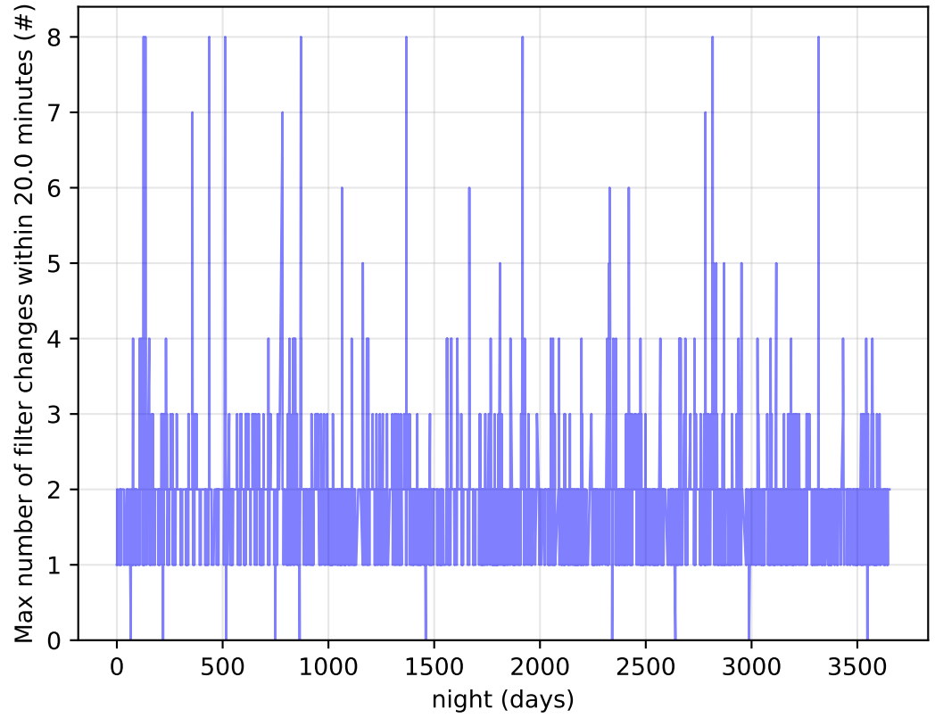
too_elab_r16_d2_ugrizyv3.4_10yrs Per Night: Max number of filter changes within 20.0 minutes
