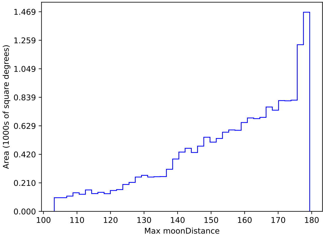
too_elab_r16_d2_ugrizy_v3.4_10yrs WFD r band: Max moonDistance
